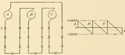
Fig. 4. Brush Multiple Circuit Arc Machine Connections
